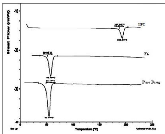
Fig 3. DSC chromatogram of pure pioglitazone, polymer (HPC) and optimized microcapsule formulation (F6).
