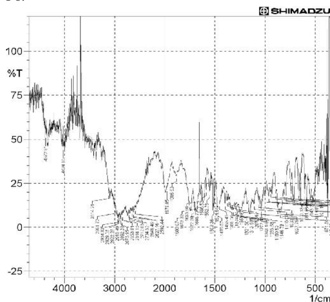
Fig 1. The FTIR data of pure drug, Pioglitazone.
