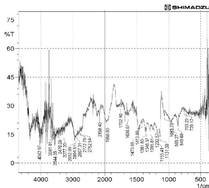
Fig 2. The FTIR data of optimized Pioglitazone microcapsule formulation (F6).
